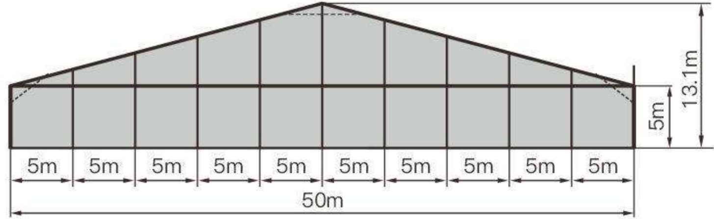
截面图 Cross Section View
