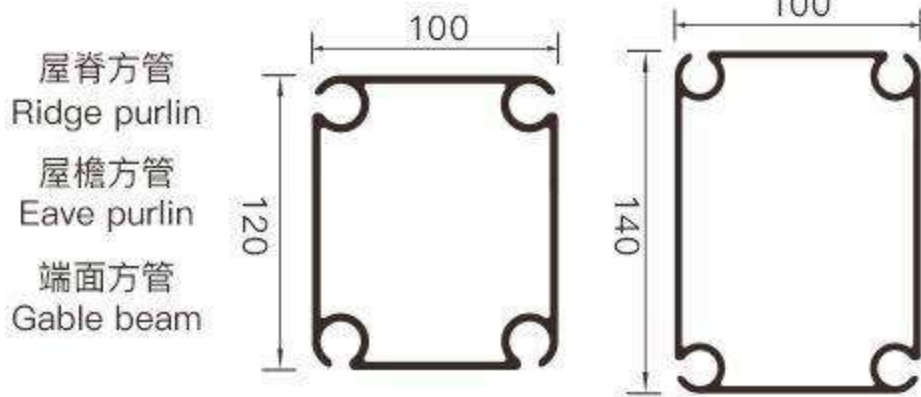
主型材尺寸 Framework Main Profile Dimension And Use
