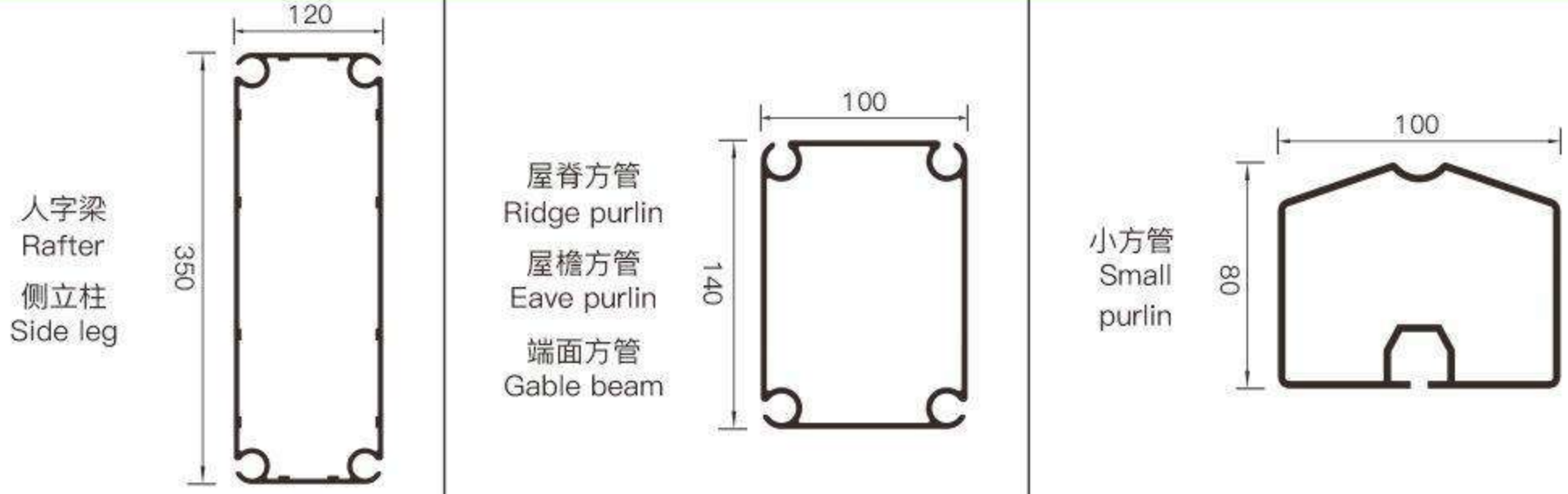
主型材尺寸 Framework Main Profile Dimension And Use
