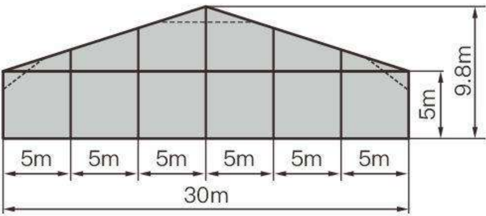
截面图 Cross Section View
